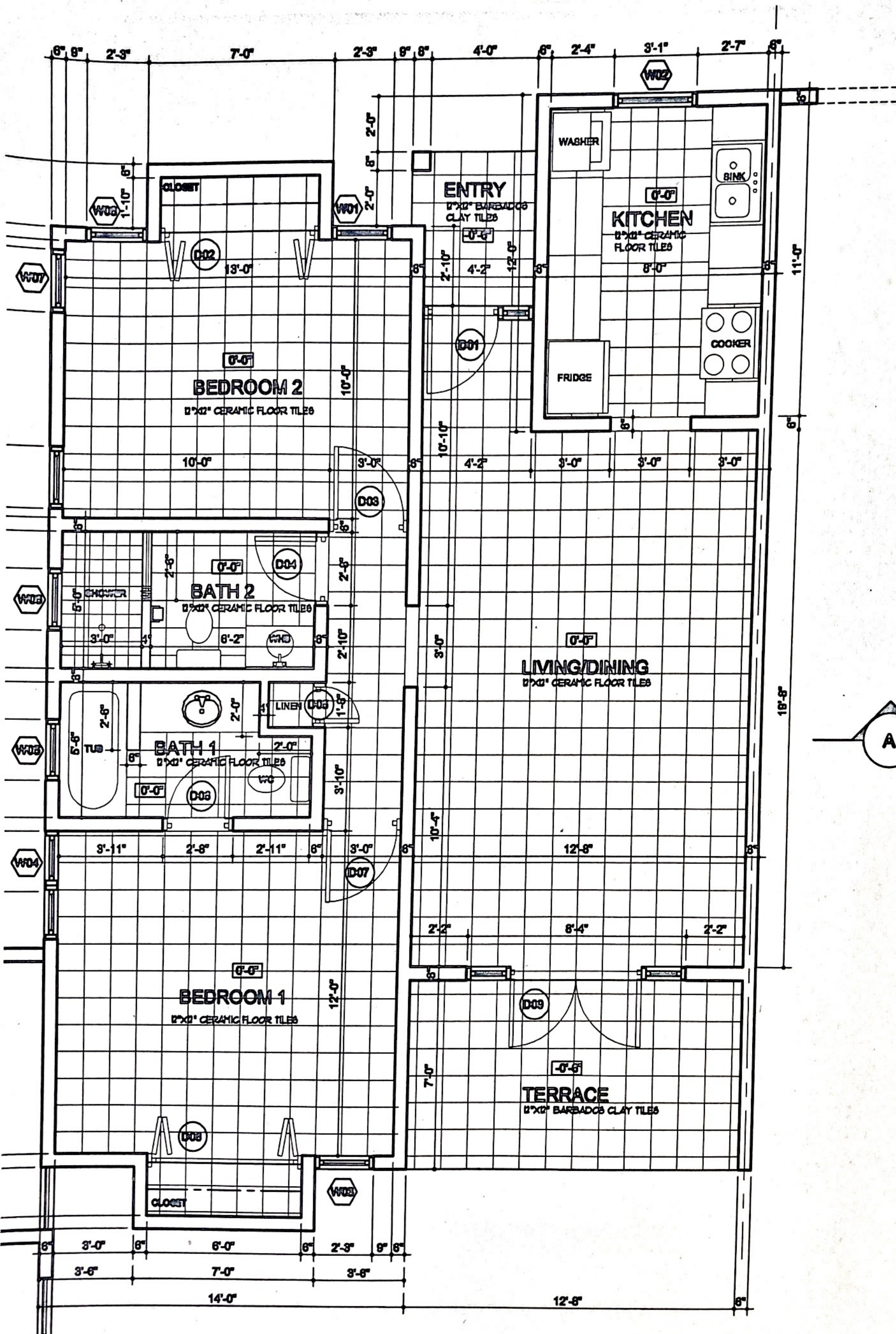
Floor Plan of D Block
